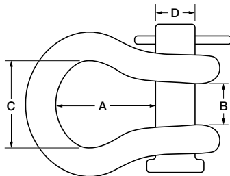
Round pin anchor shackles meet Federal Specification RR-C-271D, Type IVA Class 1, Grade A
